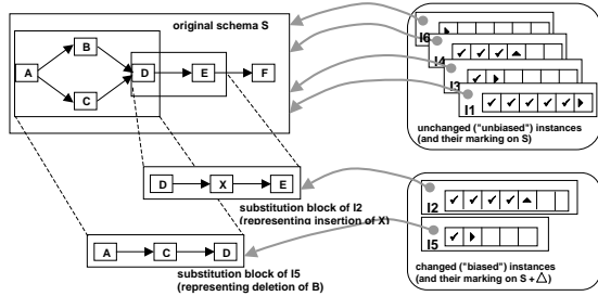
Figure 2. Managing Schema and Instance Data
