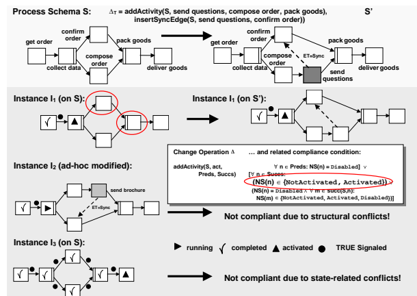
Figure 1. Migration Process (Example)
